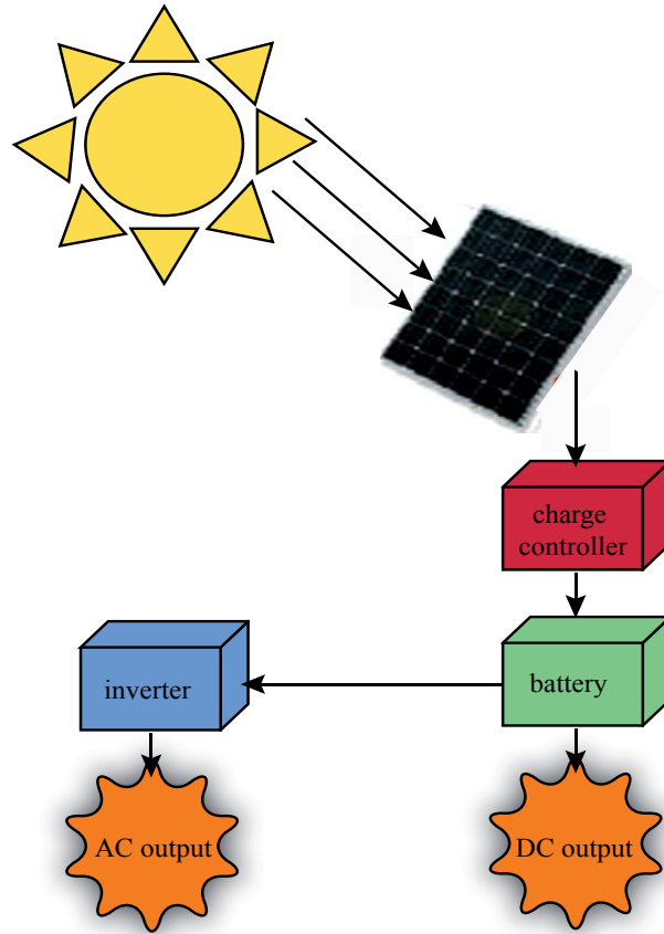
Figure 14: Photovoltaic power system
